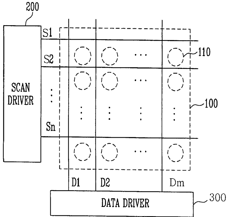
FIG. 3 RELATED ART
