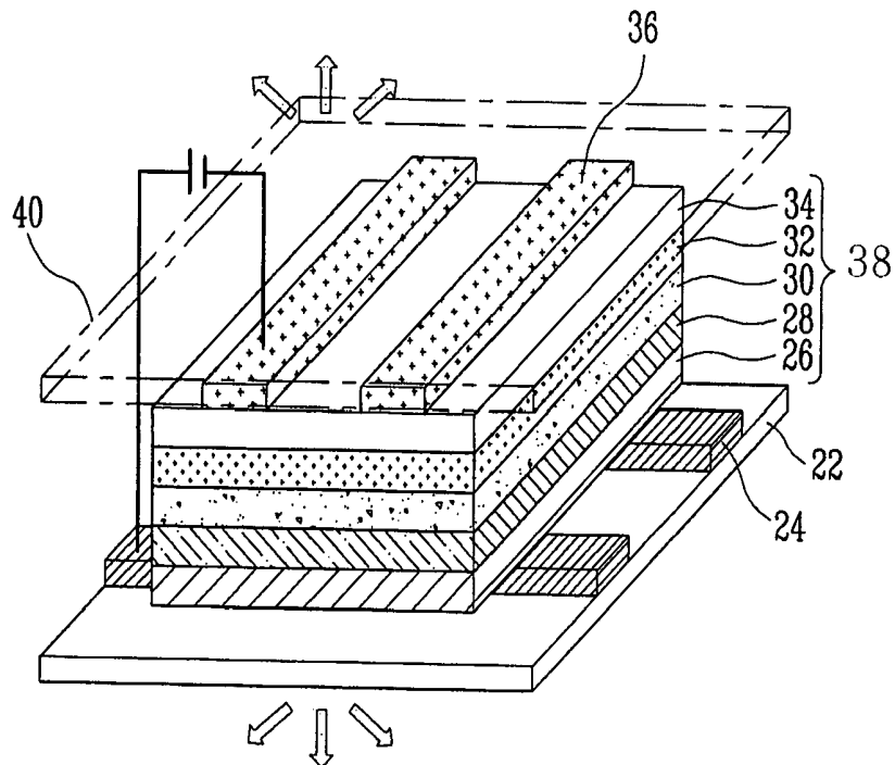
FIG. 2 RELATED ART
